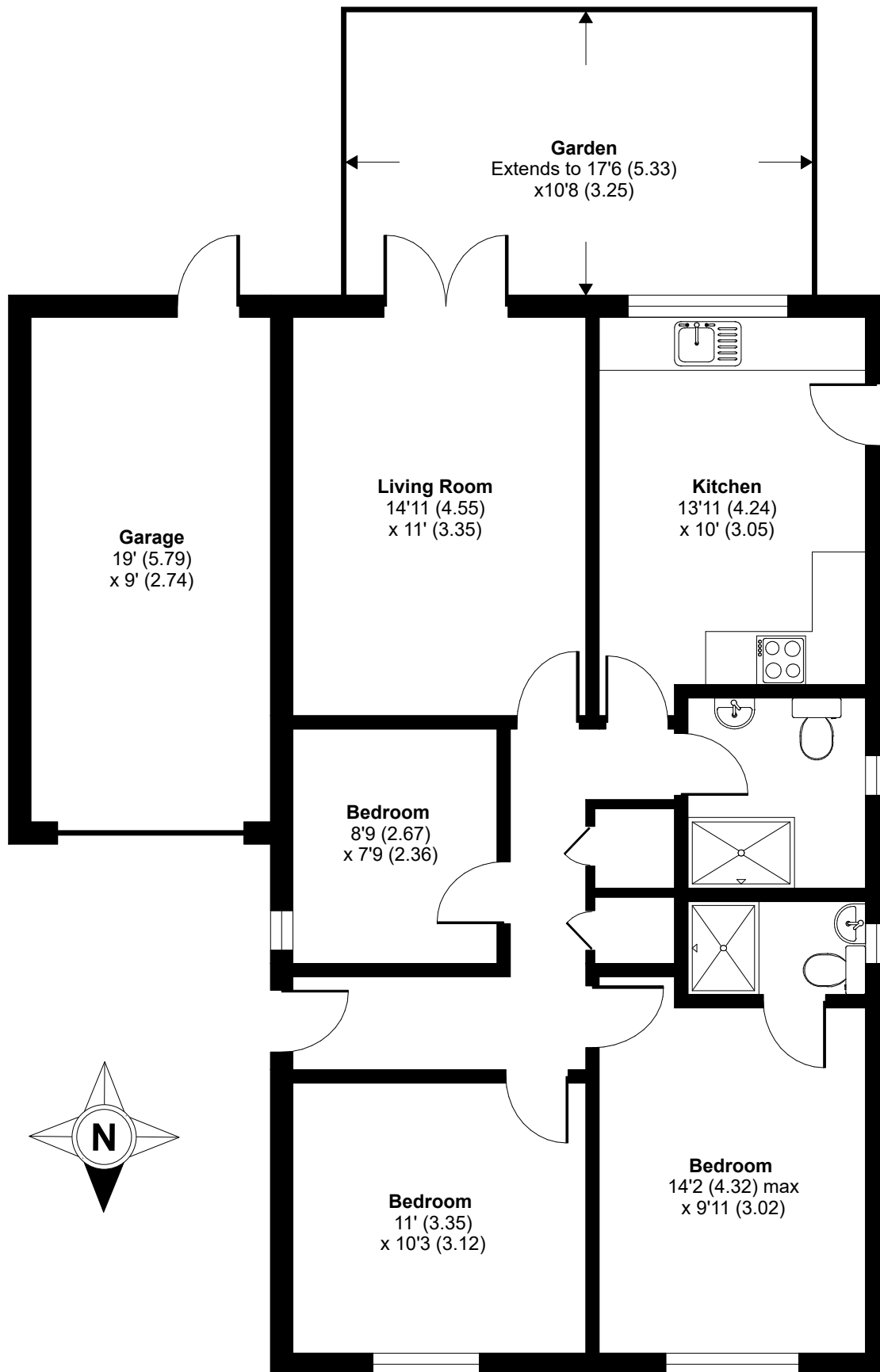
GROUND FLOOR
